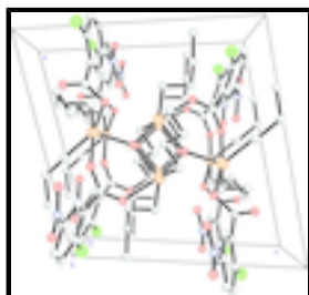
Fig. 2. The crystal structure of the title complex, viewed along the b axis, showing the title complex being stacked down the b axis. H atoms have been omitted for clarity.
